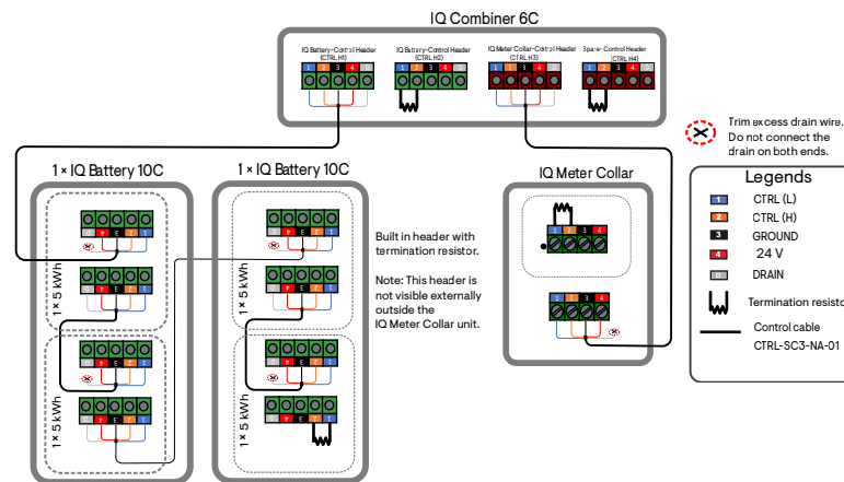
Figure 2: 1x control connector used for the battery in the IQ Combiner
