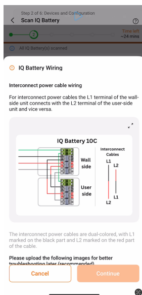
IQ Battery 10C power cable wiring
